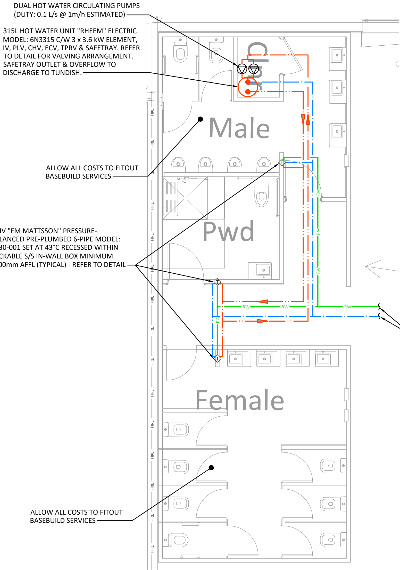
AMENITIES - TENANCY 2 SCALE 1:50
